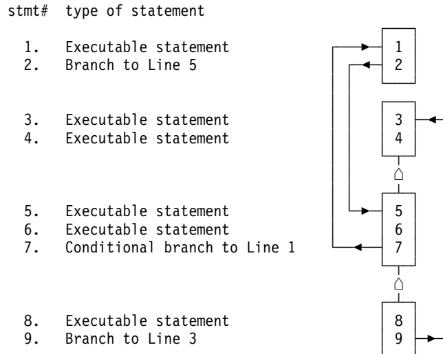
Figure 8. An example of code and nodes
