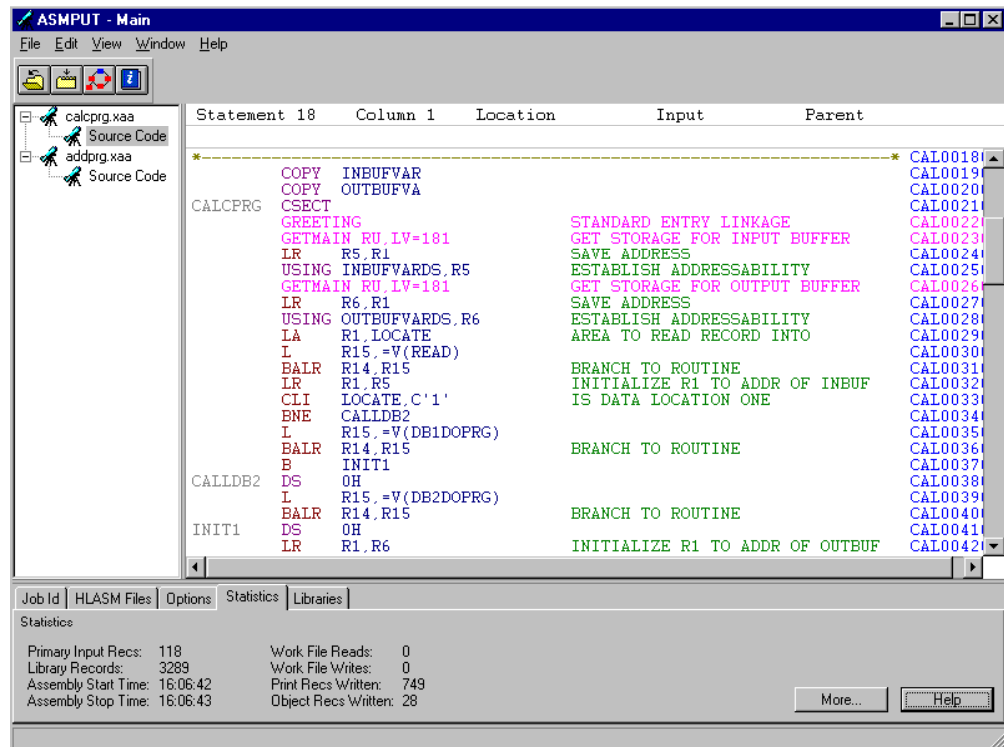
Figure 13. The information notebook Statistics tab
