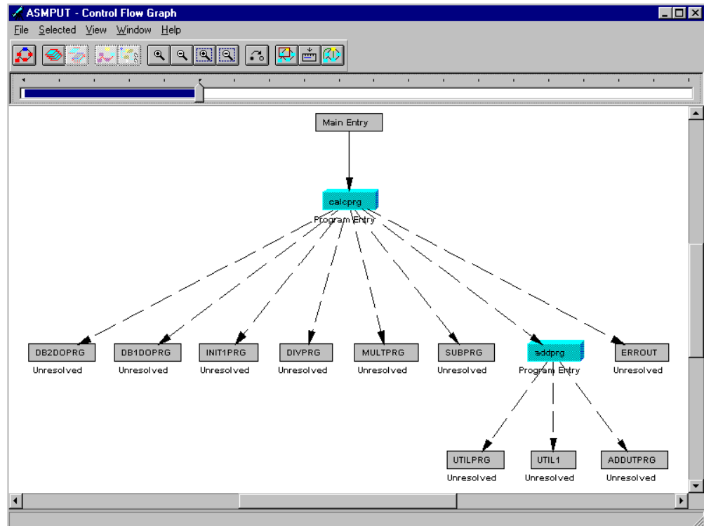
Figure 10. The ASMPUT control flow graph window
