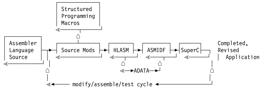
Figure 4. Toolkit Feature: Modification and Testing Phase
