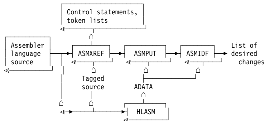
Figure 3. Toolkit Feature: Analysis and Understanding Phase
