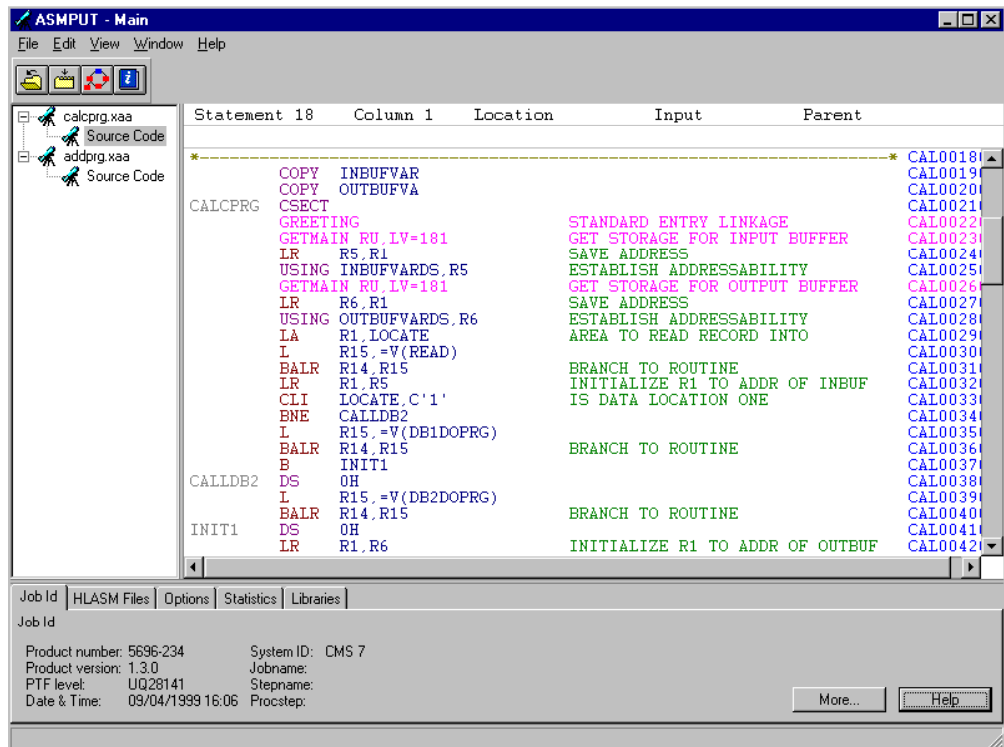
Figure 9. The ASMPUT main window
