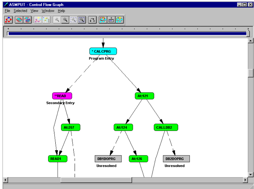
Figure 24. A graph at maximum zoom
