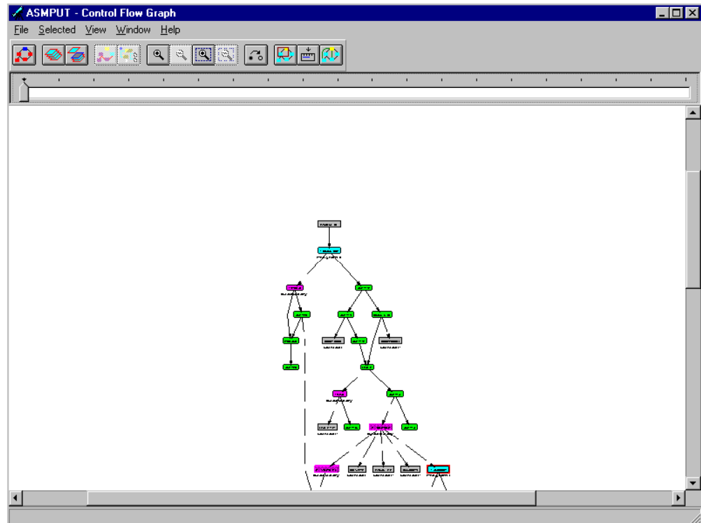
Figure 25. A graph at minimum zoom
