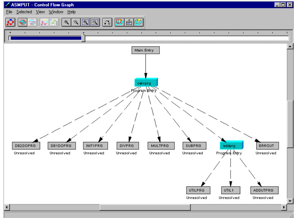
Figure 15. A completely collapsed control flow graph
