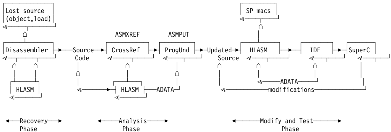
Figure 5. Toolkit Feature: Summary of Usage Phases
