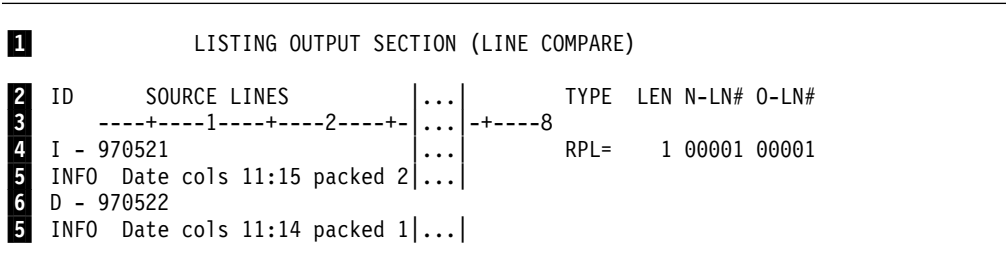
Figure 83. Example of the listing output section of the comparison listing
