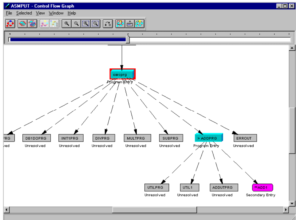
Figure 18. One node expanded in context
